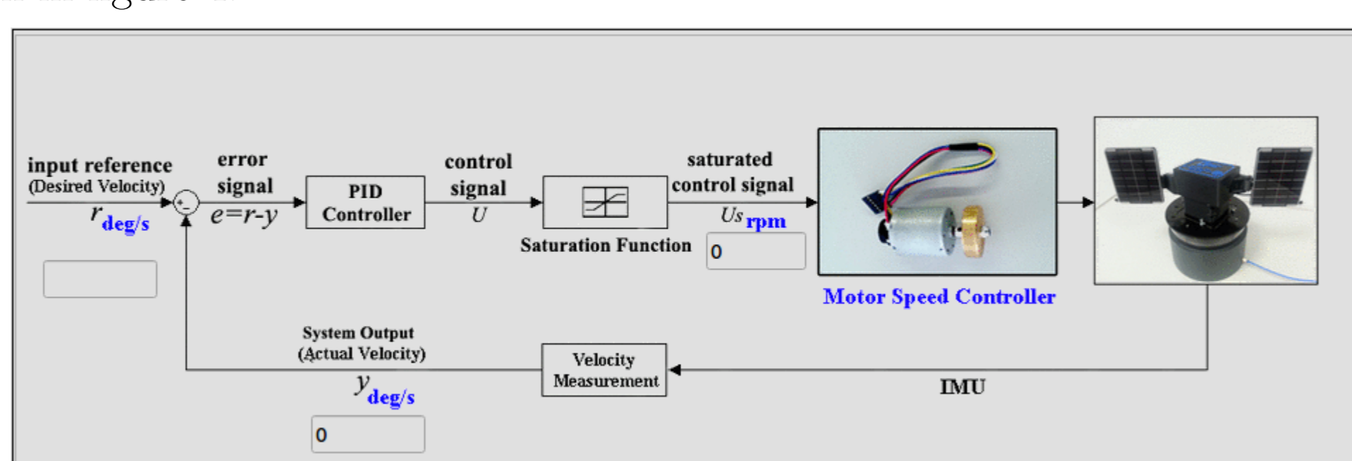
Figure 4: Velocity Controller
