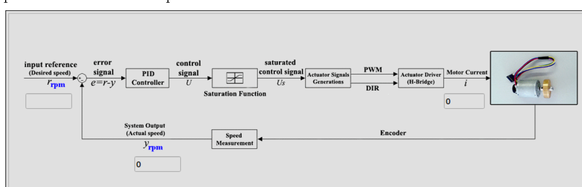
Figure 3: Motor Speed Controller
