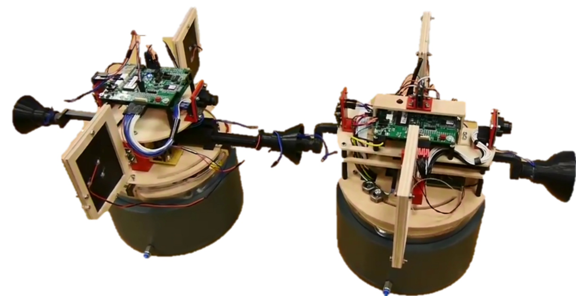
Figure 9: Display of Docking between two Float-Sats
